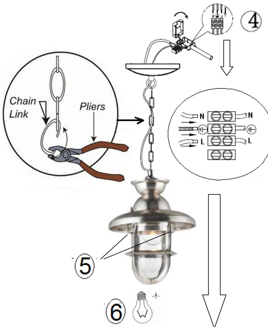
Wiring Details
